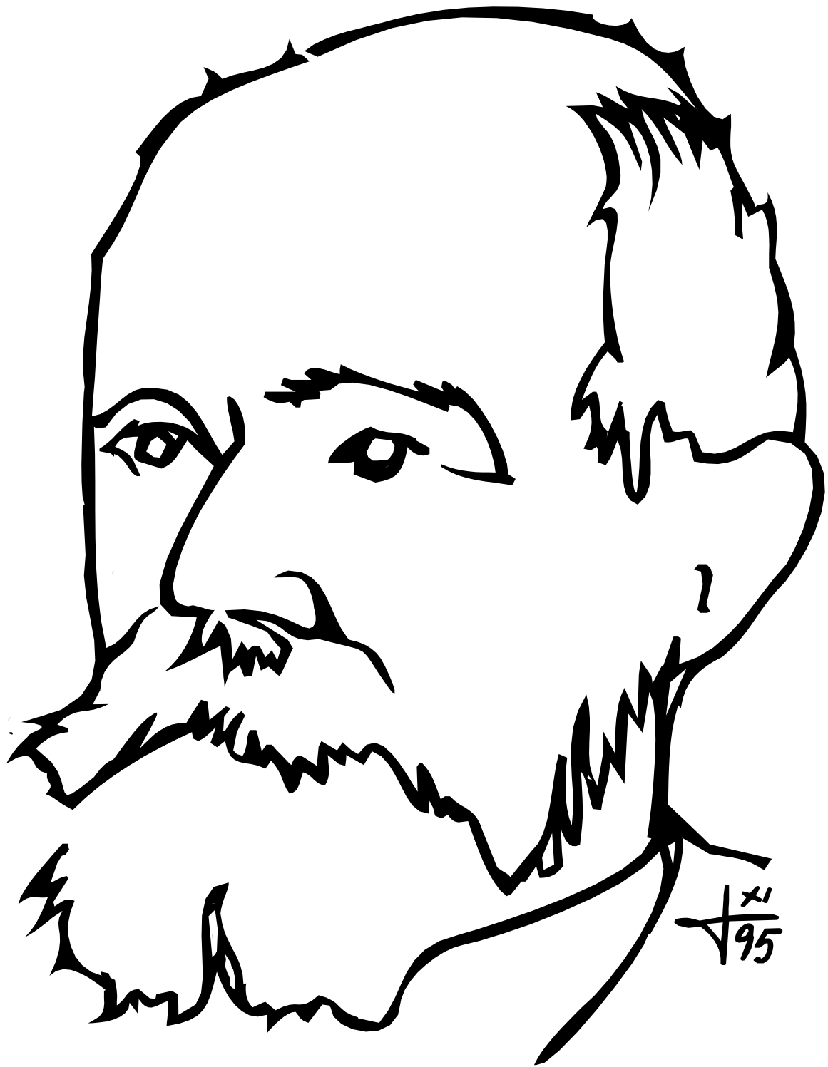
Becquerel
