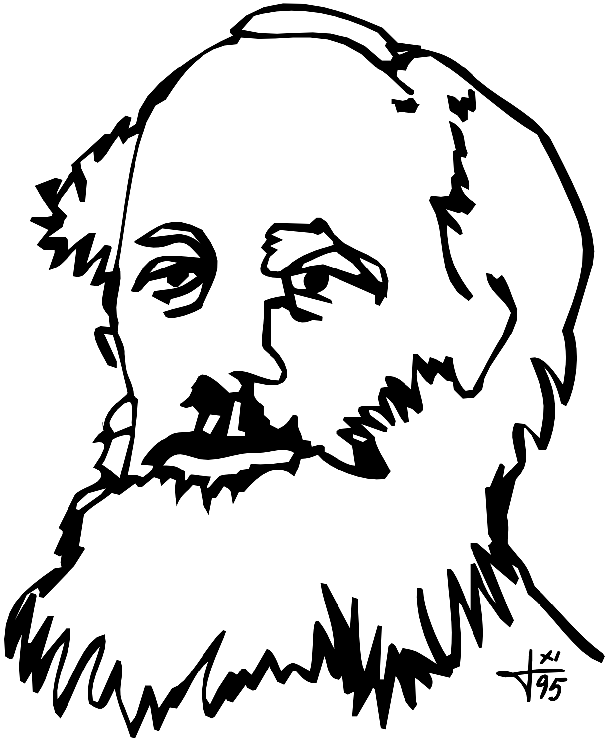
Maxwell
