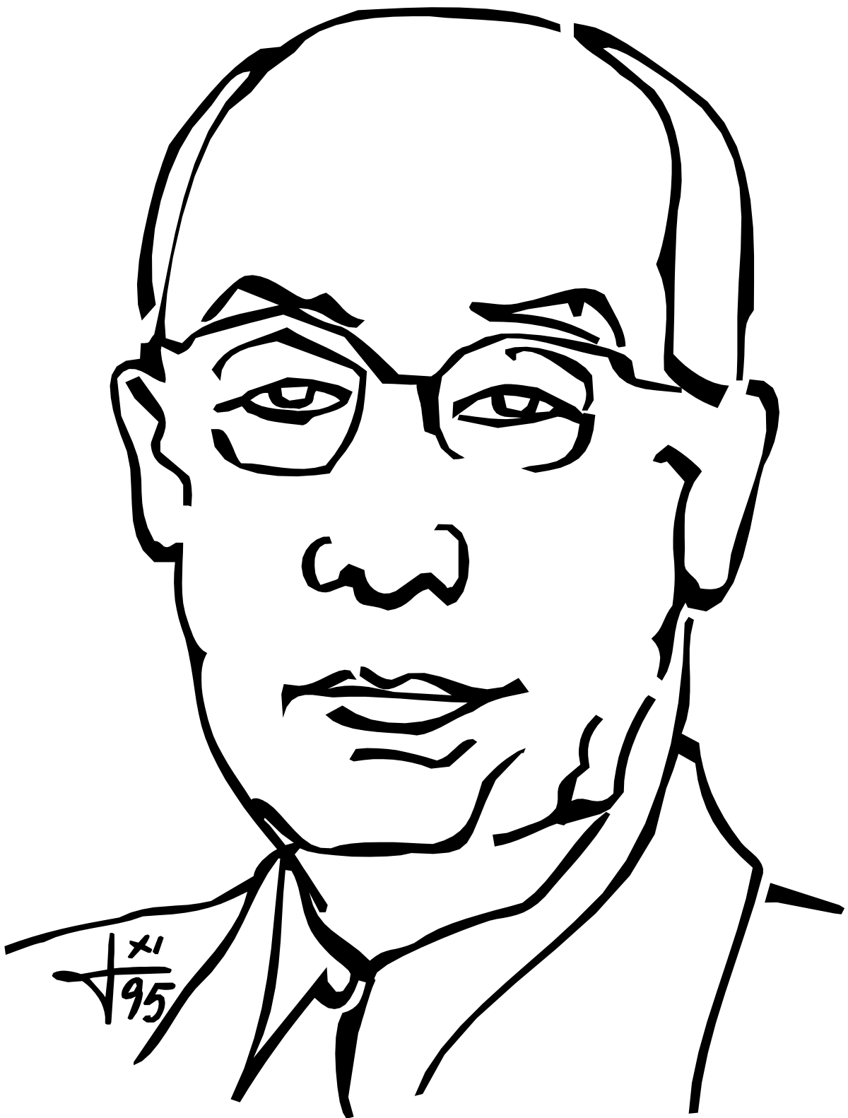
Yukawa
