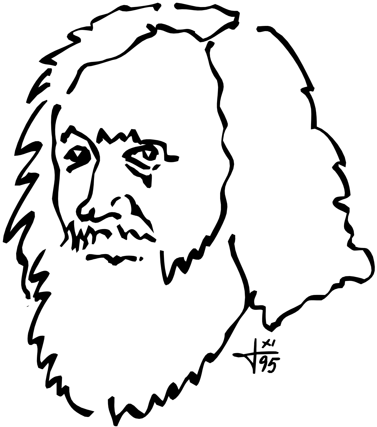
Dalton
